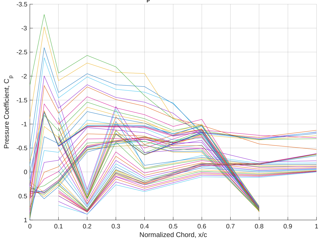
C_p vs x/c for 15 m/s
